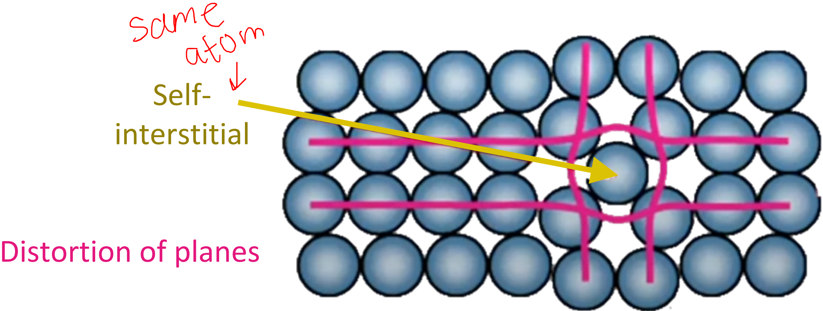
Additional atom in lattice
