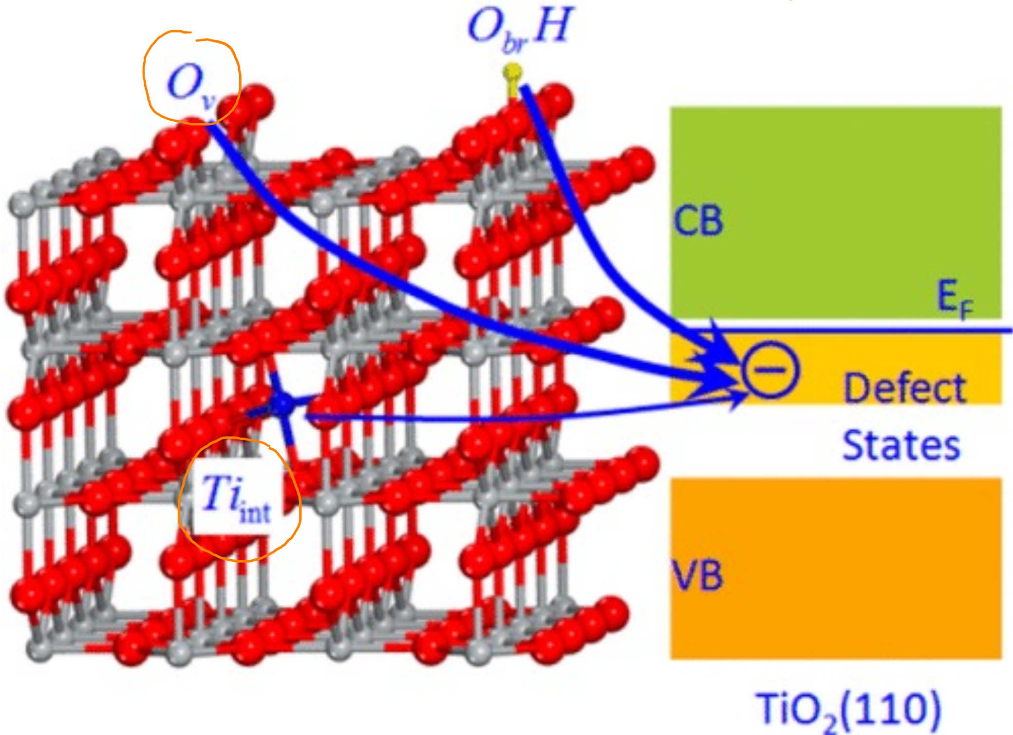
Sources of Band-Gap States of \text{TiO}_2(110)
